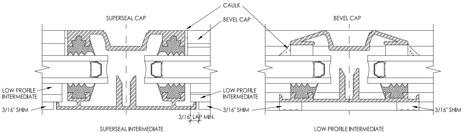
SECTION B-B
